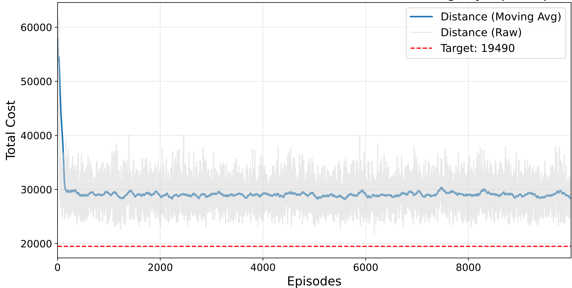
Final GAUSSIAN PROCESS Masked AutoRL-SOP Training - ry48p.3.sop
